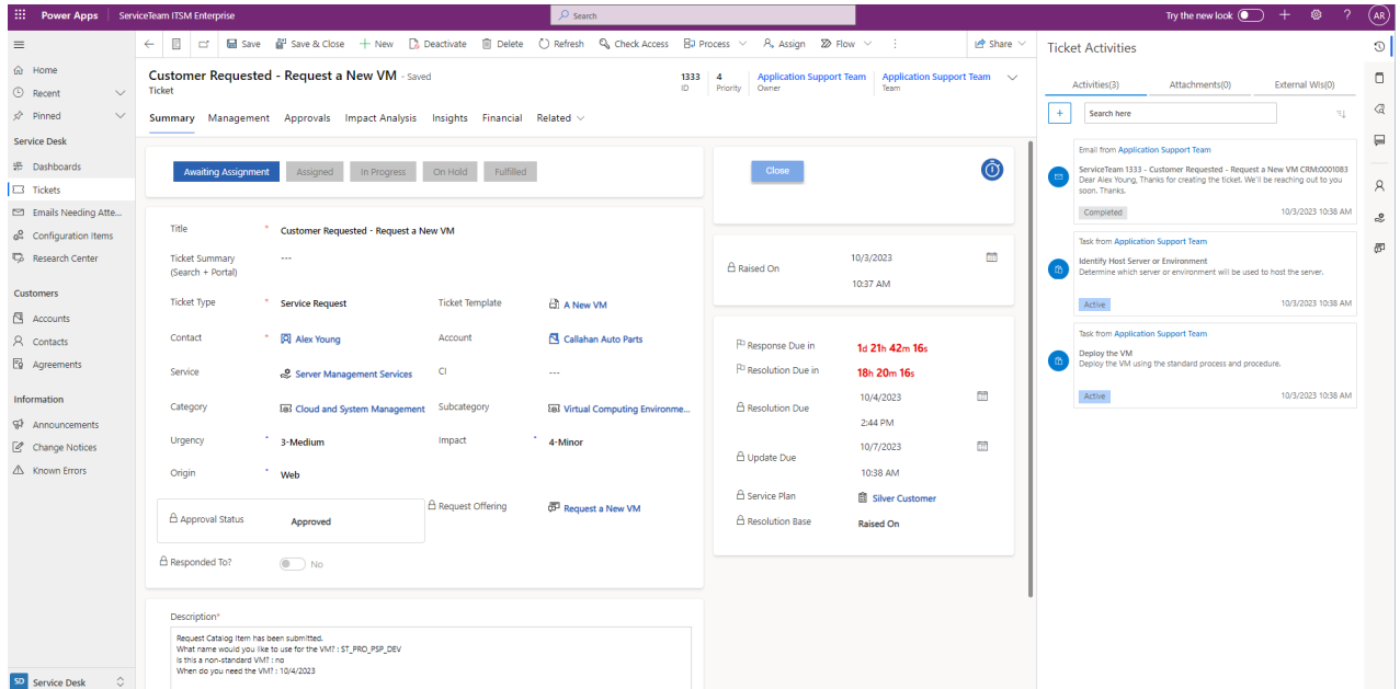
Diagram 3: The Service Desk Agent UI
